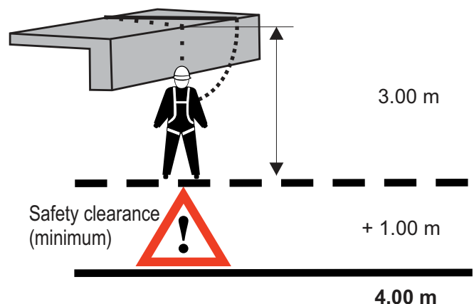
Picture 16 Lateral fall over edges
