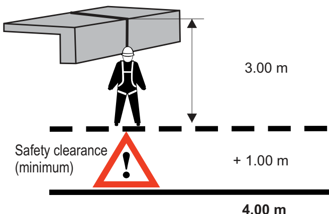
Picture 15 Rectangular fall over edges
